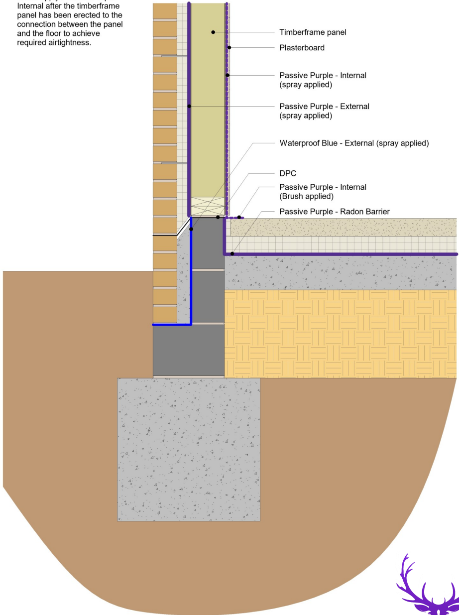
1 Timberframe - Base detail DET 7 1 : 10
